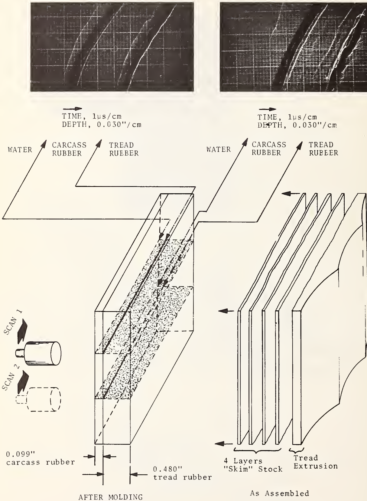
Figure 22. Carcass Rubber to Tread Interface --- B-scan Transverse to Extrusion Direction (5-MHz Transducer)
