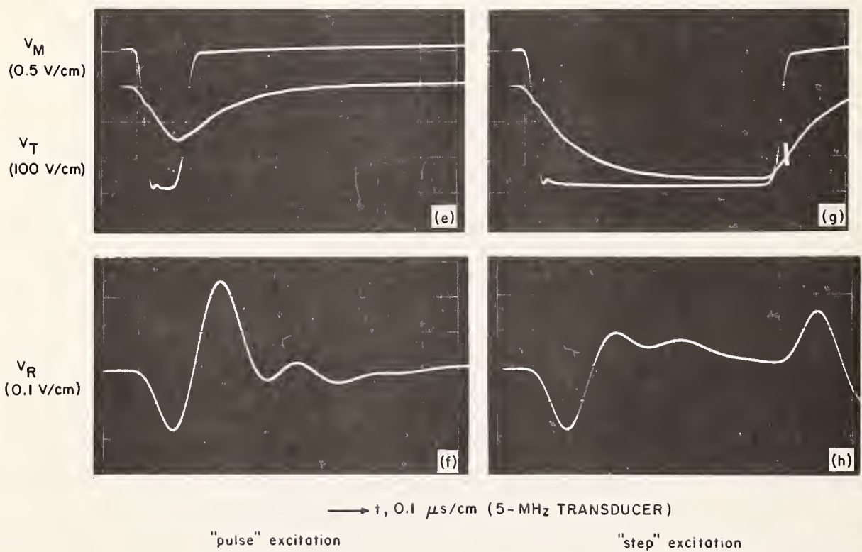
Figure 6. System Calibration Pulse Forms
