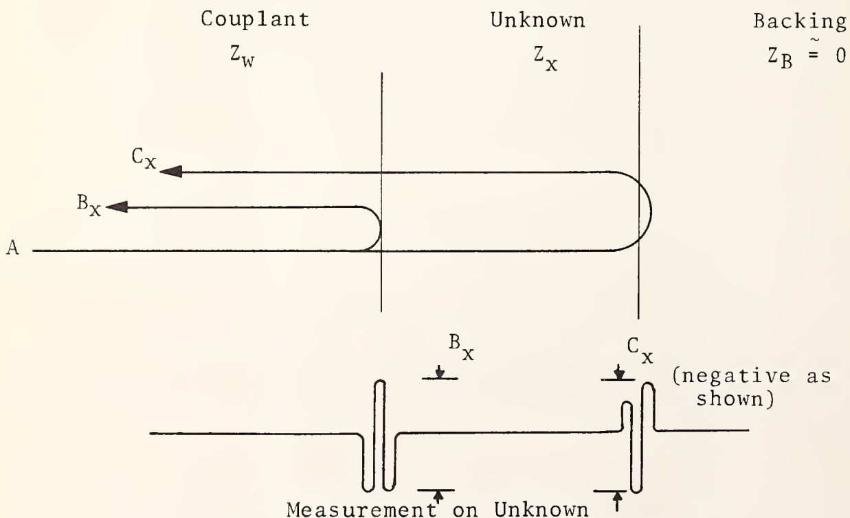
Figure A-1. Measurements on Reference Standard and Unknown
