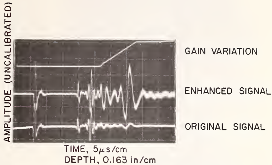
Figure 14. Time-Variation of Gain Enhancement of Reflection Signal (5-MHz Transducer)
