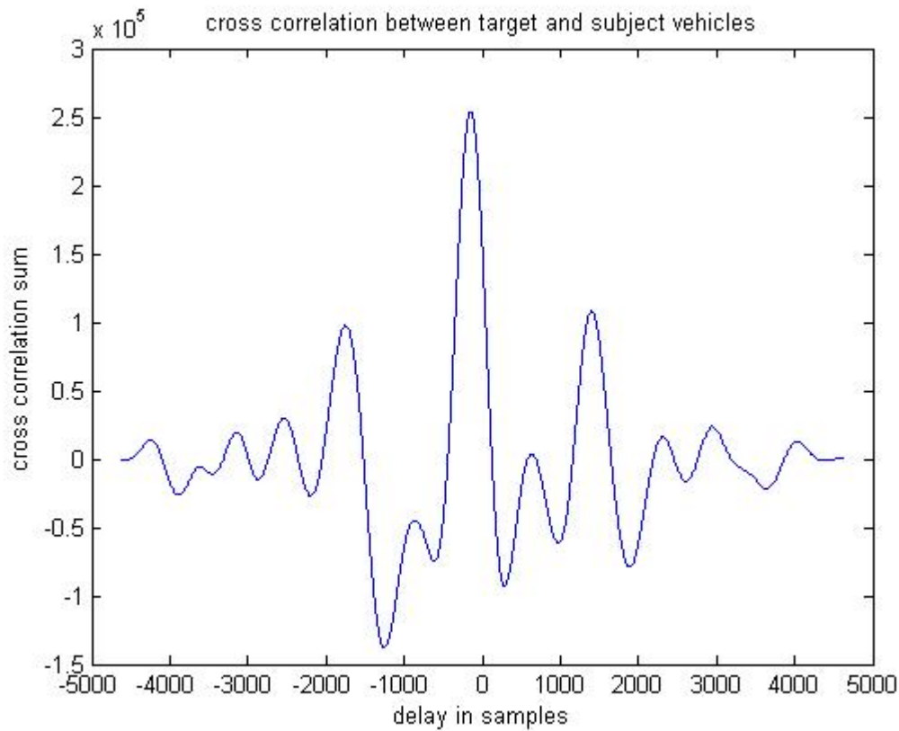
Figure 28. Cross Correlation between Subject and Lead Vehicles
