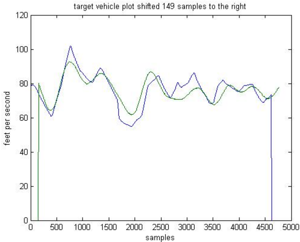
Figure 29. Peak of Cross Correlation Function (Offset of -149 Samples)
