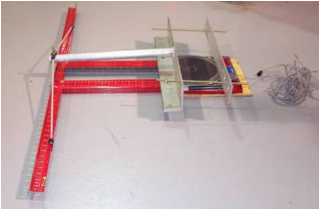
Figure 6. Apparatus for Recording Steering Wheel Movement
