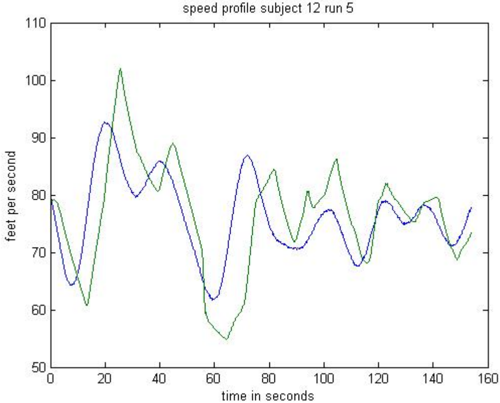
Figure 27. Sample Speed Trace of Subject Vehicle Following the Lead Vehicle
