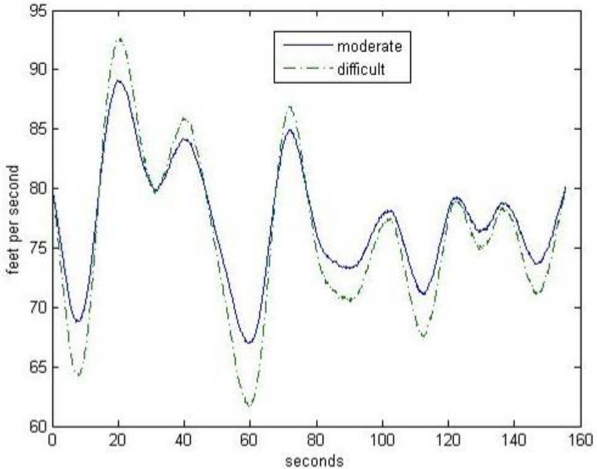
Figure 1. Lead Vehicle Car-Following Speed Signals – Experiment 1
