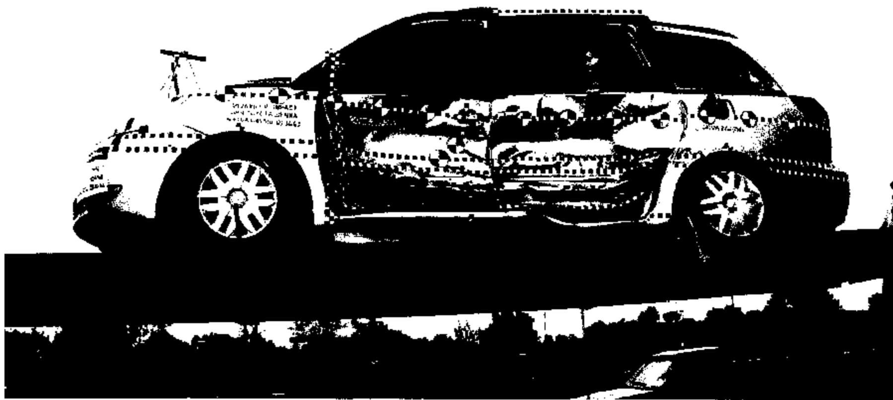
Figure A-46 ROLL OVER 360 DEGREES
