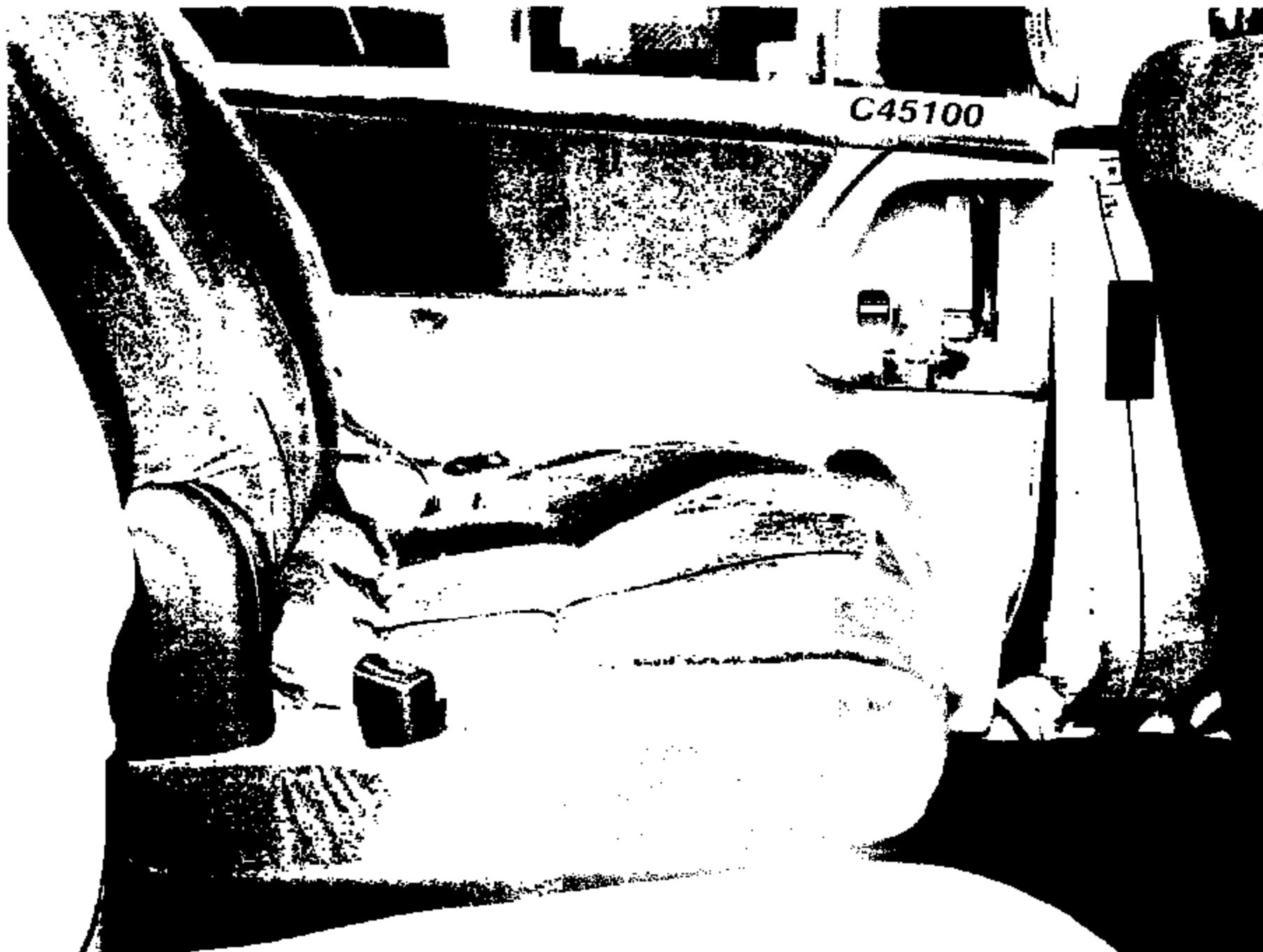
Figure A-36 POST-TEST INTERIOR OF REAR DOOR SHOWING SIDE IMPACT LOCATIONS
