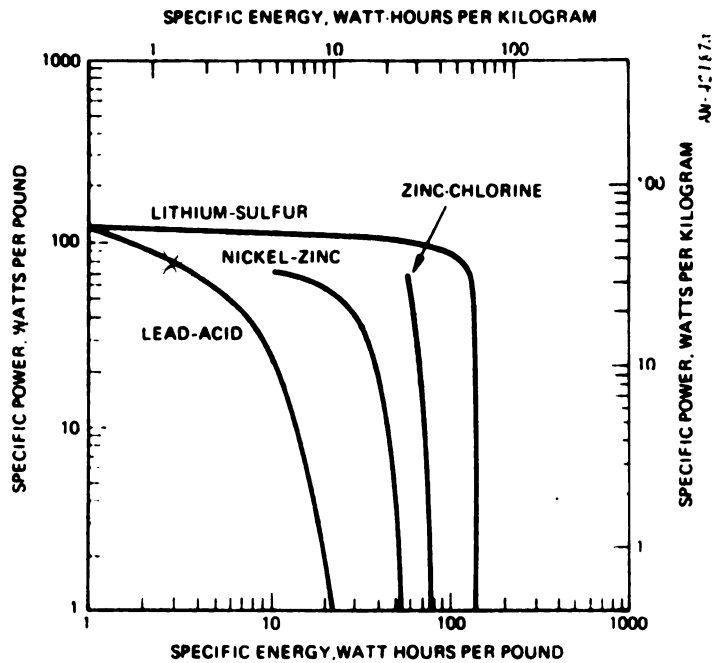
Figure 2.1. Assumed Battery Capabilities (Source: Task Report 1, Fig. 5.15)
