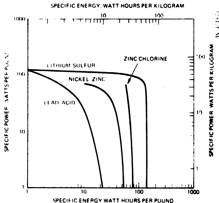
Figure 1.1. Assumed Battery Capabilities
