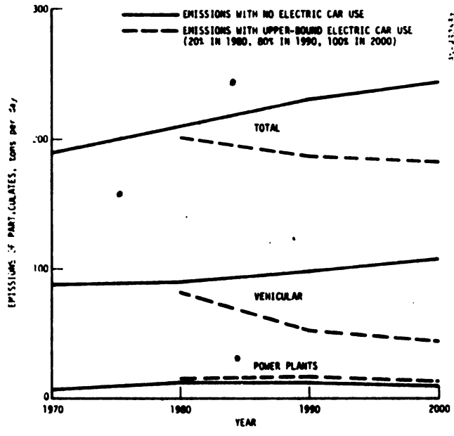
Figure 4.8. Projected Particulate Emissions (Source: Task Report 7, Fig. 3.6)
