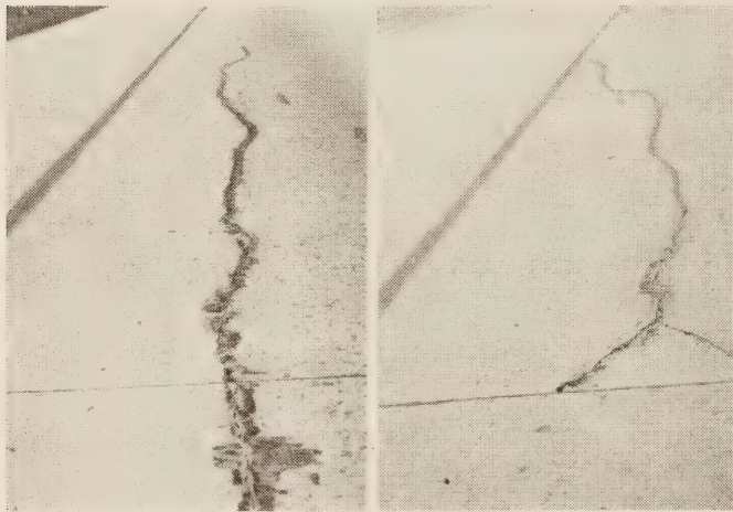
FIGURE 6.—TYPICAL LONGITUDINAL CRACKS OBSERVED IN 1944 IN INDIANA PAVEMENT SN-FA 13-B (2).
