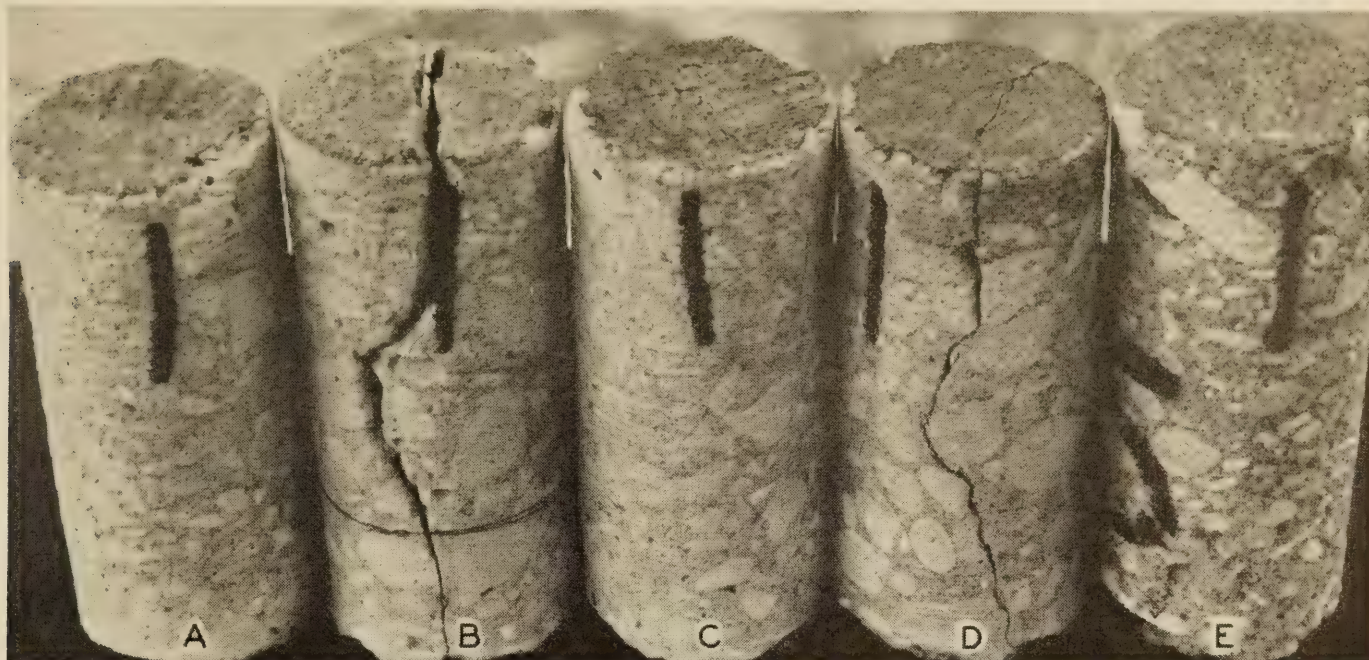
FIGURE 9.—TYPICAL CORES DRILLED AT THE LONGITUDINAL JOINT IN THE 1942 ILLINOIS PAVEMENTS.
