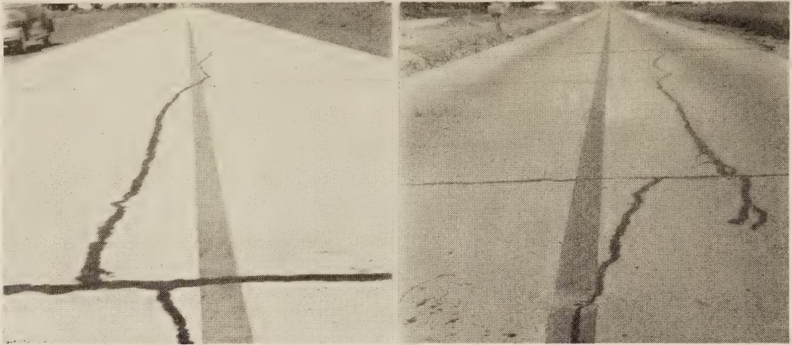
FIGURE 10.—TYPICAL LONGITUDINAL CRACKS IN THE 1942 PAVEMENTS OF ILLINOIS.
