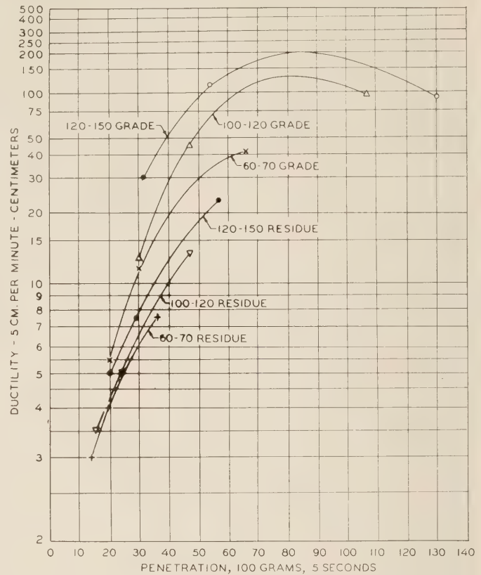
FIGURE 3.—RELATION BETWEEN DUCTILITY AND PENETRATION FOR SAMPLE 8.
