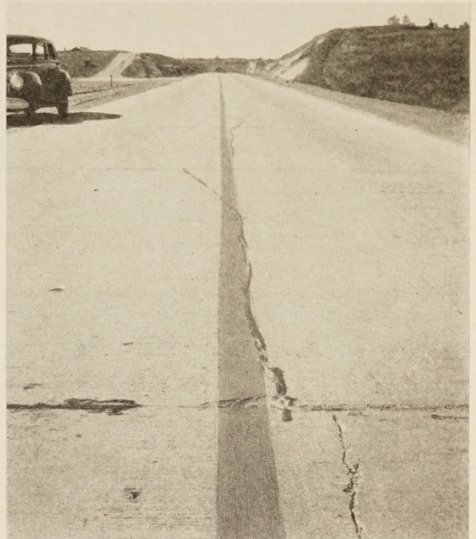
FIGURE 1.—LONGITUDINAL CRACK IN SECTION OF PAVEMENT WHERE THE CENTER JOINT HAS NOT CRACKED.
