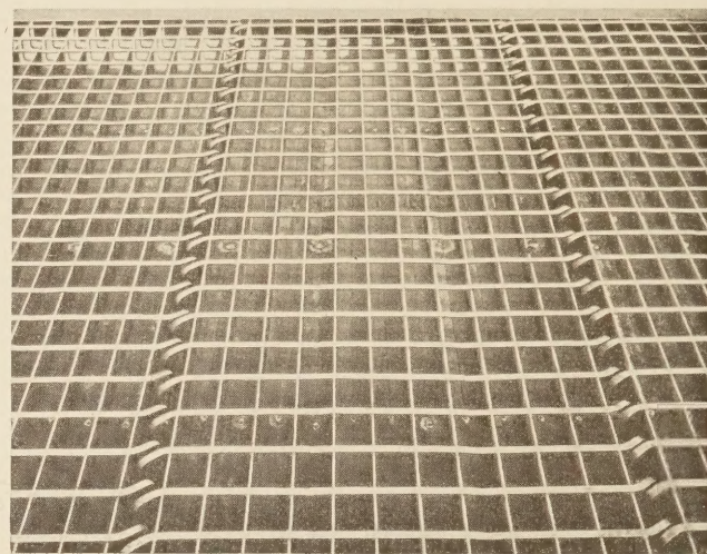
FIGURE 5.—COMPLETED MAT USED IN CONSTRUCTION OF SECOND SLAB BEFORE BEING FILLED WITH CONCRETE. NOTE NUMBER AND POSITION OF WELDS AND ALSO METHOD USED FOR UNITING EDGES OF INDIVIDUAL MATS
