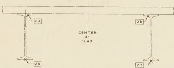
FIGURE 8.—LOCATIONS OF STRAIN-GAGE POINTS
