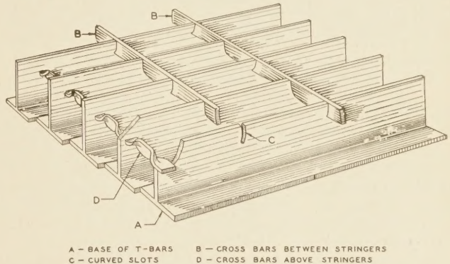
FIGURE 2.—ASSEMBLY OF STEEL SECTION OF FIRST SLAB
