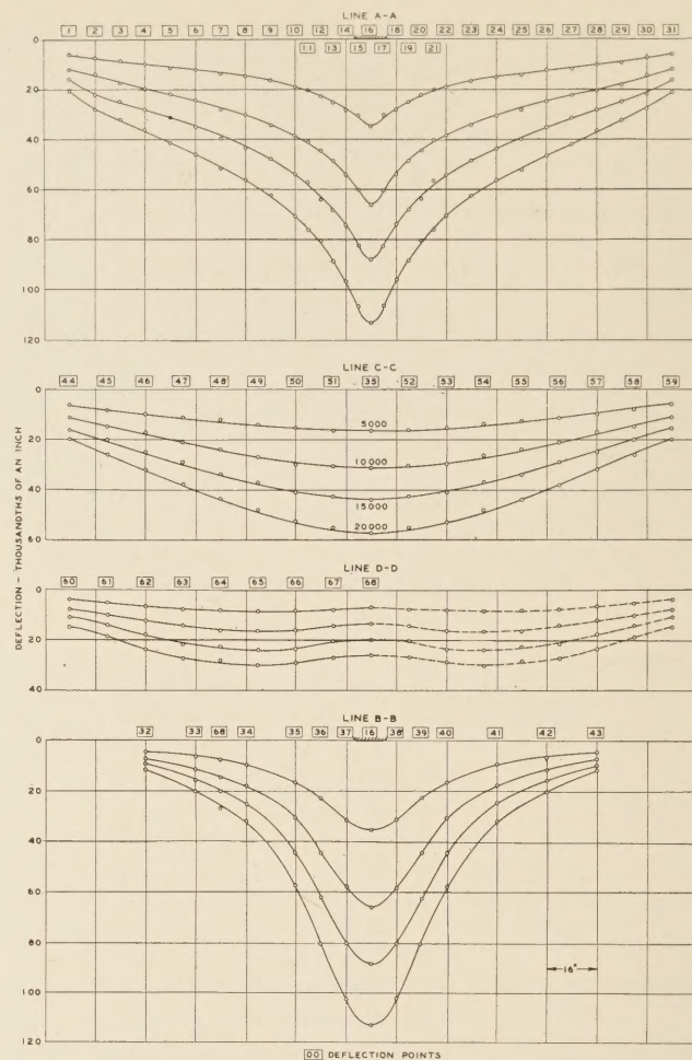
FIGURE 16.—DEFLECTIONS OF FIRST SLAB UNDER CENTER LOADING AFTER FIRST IMPACT
