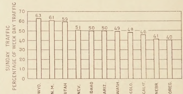
FIGURE 7.—COMPARISON OF SUNDAY AND WEEK-DAY TRUCK TRAFFIC
