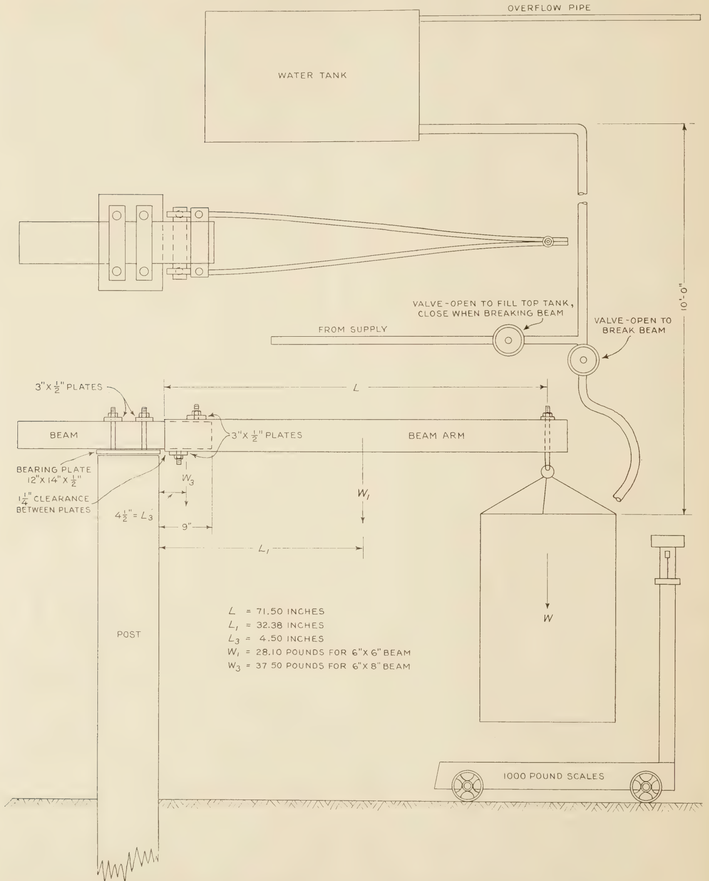
FIGURE 1.—DIAGRAM OF IMPROVISED SINGLE-LEVER FIELD MACHINE AS USED IN TESTS
