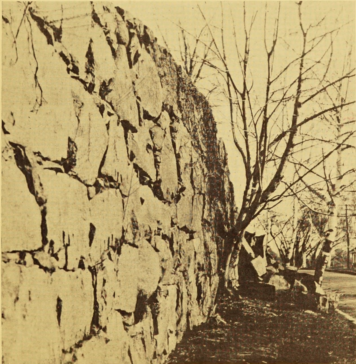
FAILURE OF A PORTION OF A RETAINING WALL
