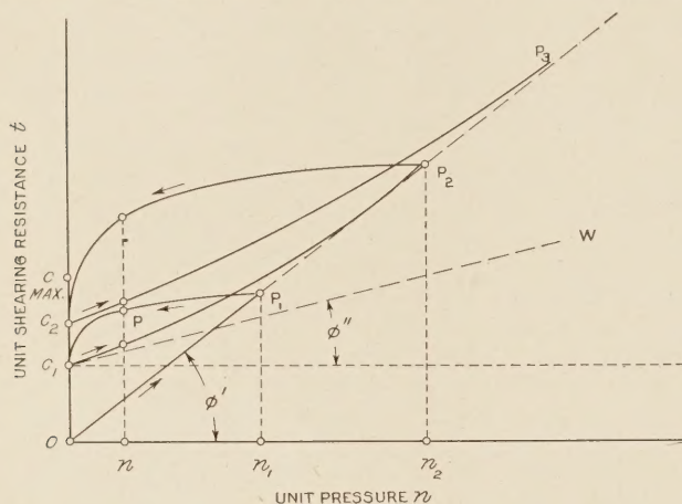
FIGURE 4.—RELATION BETWEEN PRESSURE PER UNIT OF AREA, n , AND RESISTANCE PER UNIT OF AREA AGAINST DISPLACEMENT, t
