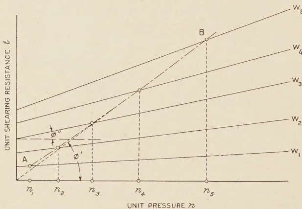
FIGURE 5.—RELATION BETWEEN n AND t ACCORDING TO DR. H. KREY
