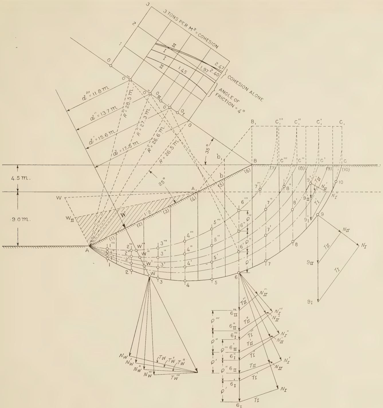
FIGURE 15.—DIAGRAM USED IN SOLUTION OF TYPICAL STABILITY PROBLEM
