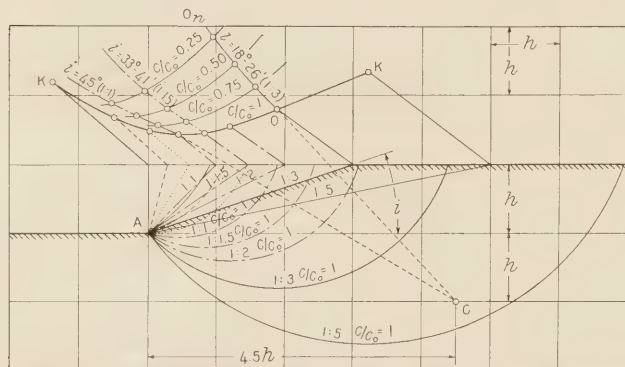
FIGURE 10.—DIAGRAM SHOWING METHOD OF LOCATING CENTER OF SLIDING CURVE
