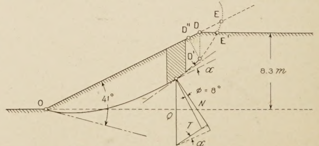
FIGURE 7.—SLIDING CURVE DERIVED BY FRONTARD'S METHOD
