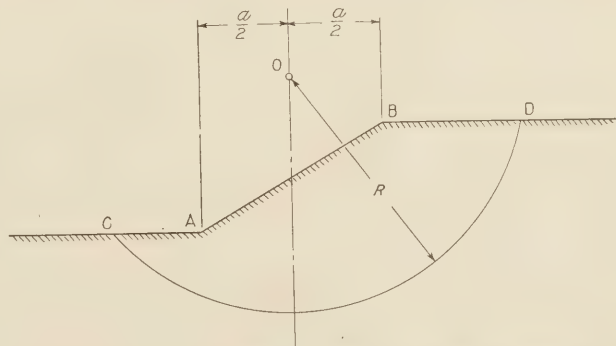
FIGURE 9.—SHAPE OF MOST DANGEROUS SLIDING SURFACE ON SLOPES OF LESS THAN 53°
