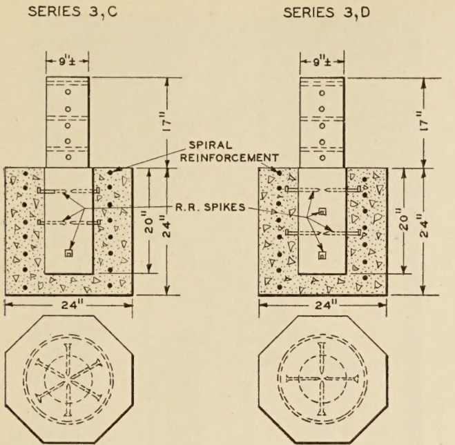
SERIES 3, C.—SIX RAIL SPIKES \frac{5}{8} BY 6 INCHES, DRIVEN AS SHOWN SERIES 3, D.—EIGHT RAIL SPIKES \frac{5}{8} BY 6 INCHES, DRIVEN AS SHOWN
