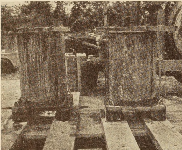
ANCHORAGE SPECIMENS SHOWING PILE ENDS FLUSH WITH SURFACE OF CONCRETE (TOP PICTURE) AND SPECIMENS READY FOR CURING UNDER WATER
