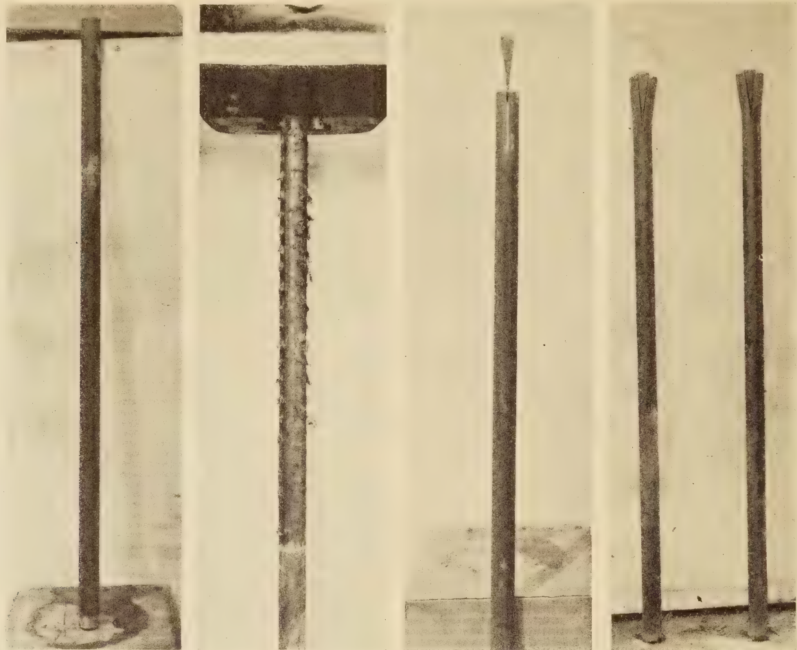
PICTURES TAKEN IN ORDER FROM THE LEFT SHOW A HACKED BAR USED IN SERIES 4,A BEFORE DRIVING; ONE OF THESE BARS PULLED FROM A PILE WITH WOOD FIBER ON HACKS; A FOX BOLT OF SERIES 5 BEFORE DRIVING, AND TWO OF THESE BARS PULLED FROM A PILE HEAD SHOWING COMPLETE EXPANSION OF THE ENDS
