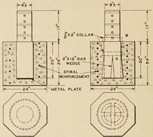
SERIES 1.—PLAIN BOND, CONCRETE PLACED IN AIR SERIES 7.—SAME AS SERIES 1, EXCEPT END BOND PREVENTED BY THIN METAL PLATE SERIES 8.—SAME AS SERIES 1, EXCEPT CONCRETE PLACED UNDER WATER SERIES 2.—PILE HEAD EXPANDED WITH OAK WEDGES, STEEL COLLAR PLACED IN PILE AT A, WHILE WEDGES WERE DRIVEN, THEN MOVED TO B WHILE CONCRETE WAS PLACED, AND REMOVED ENTIRELY BEFORE TESTING
