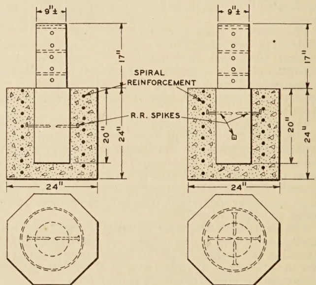
SERIES 3, A.—TWO RAIL SPIKES 5/8 BY 6 INCHES, DRIVEN AS SHOWN SERIES 3, B.—FOUR RAIL SPIKES 5/8 BY 6 INCHES, DRIVEN AS SHOWN
