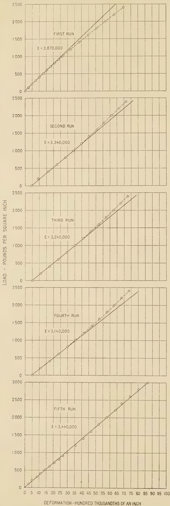
FIG. 3.—LOAD-DEFORMATION CURVES OF A 1:2:3 CONCRETE CYLINDER UNDER REPEATED LOADING
