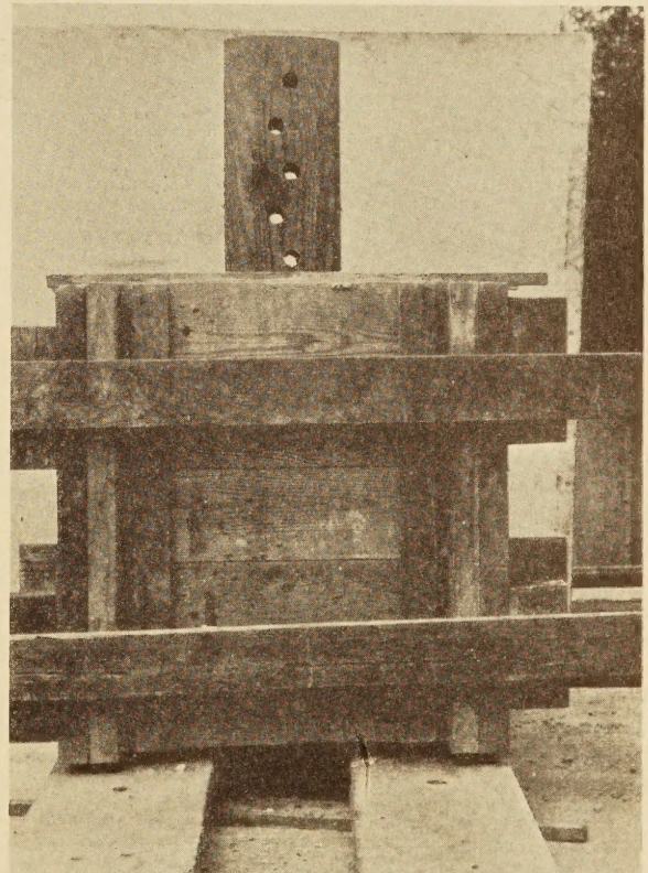
PILE SECTION ENCASED IN CONCRETE BEFORE THE REMOVAL OF THE FORMS
