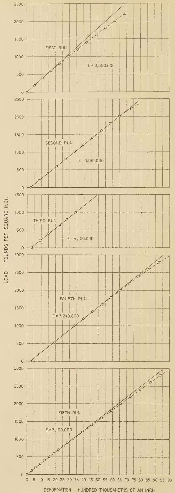
FIG. 4.—LOAD-DEFORMATION CURVES OF A 1:2 MORTAR CYLINDER UNDER REPEATED LOADING
