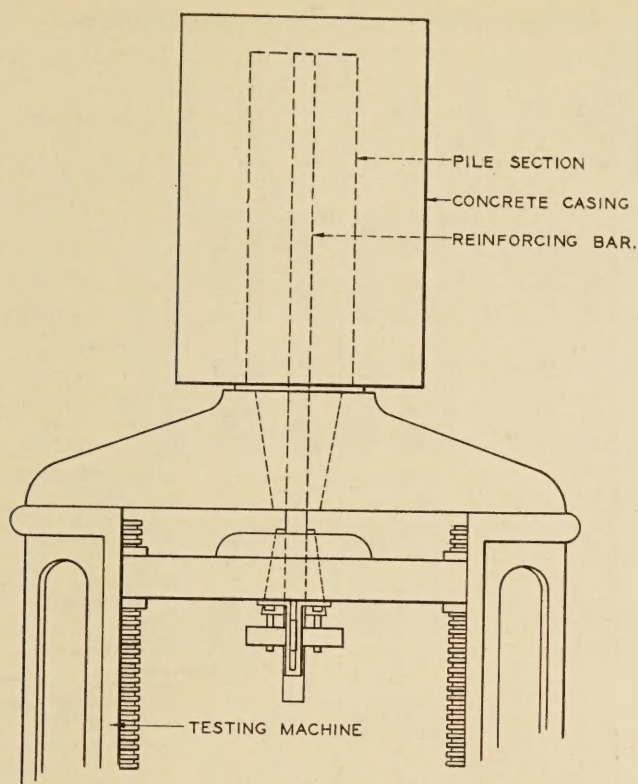
FIG. 6.—APPARATUS USED IN ANCHORAGE TESTS
