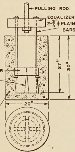
SERIES 6.—PILE HEAD EXPANDED WITH OAK WEDGES. REINFORCING BARS HOOKED UNDER STEEL COLLAR
