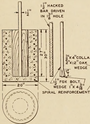
SERIES 4, A.—HACKED BAR USED SERIES 4, B.—SMOOTH BAR USED SERIES 5.—FOX BOLT USED
