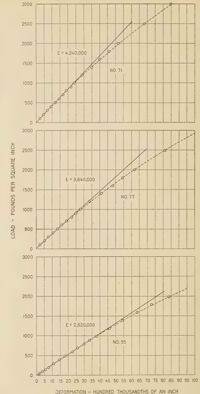
FIG. 1.—TYPICAL LOAD-DEFORMATION CURVES FOR MORTAR SPECIMENS. DEFORMATIONS SHOWN ARE PER INCH OF LENGTH
