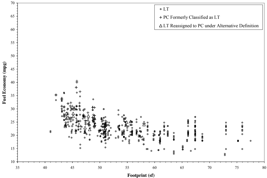
Figure XI-2. Effect on the MY 2011 Light Truck Fleet
