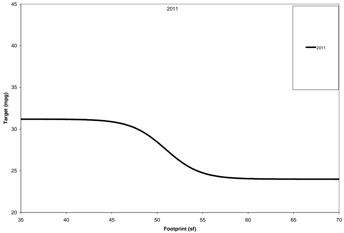
Figure IX-1. Passenger Car Curve Target Function
