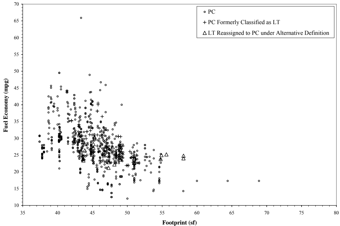
Figure XI-1. Effect on the MY 2011 Passenger Car Fleet
