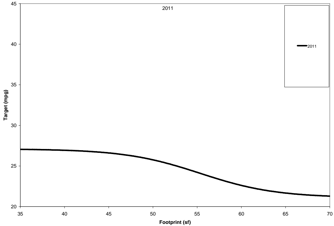
Figure IX-2. Light Truck Curve Target Function
