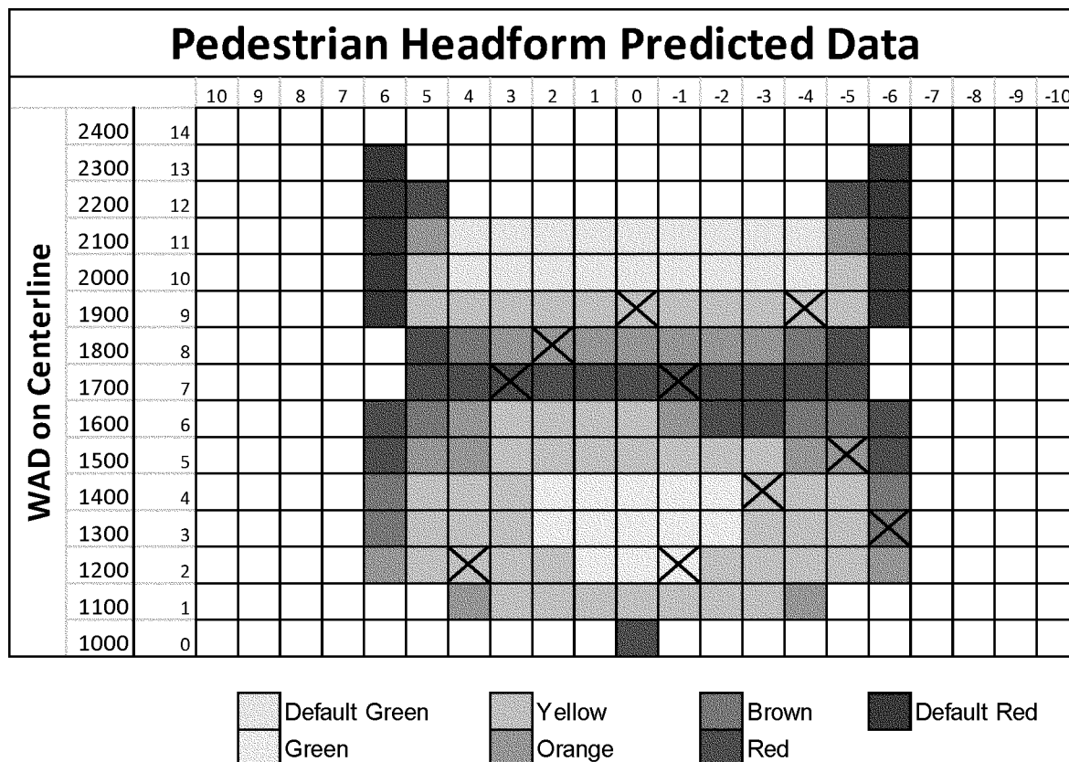
Figure 17: Example of Manufacturer's Predicted Head Impact Data
