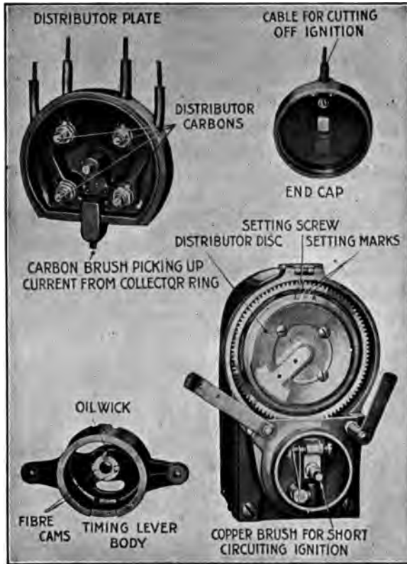
FIG. 222.—Principal parts of Eisemann high-tension magneto, type G4, I Edition.
