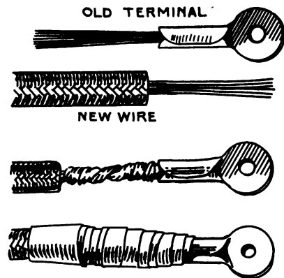
FIG. 328.—Method of using old terminals on new wires.
