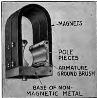
FIG. 204.—Magnets and pole pieces of Bosch magneto.
