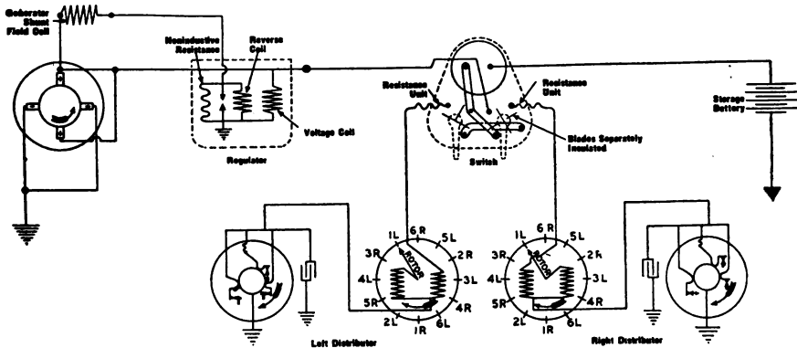
FIG. 177.—Circuit diagram of Liberty Twelve aircraft engine ignition system.
