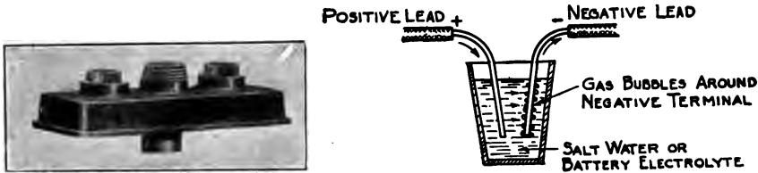
FIG. 50.—Cover for battery cell. FIG. 51.—Method of determining polarity of storage battery terminals.
