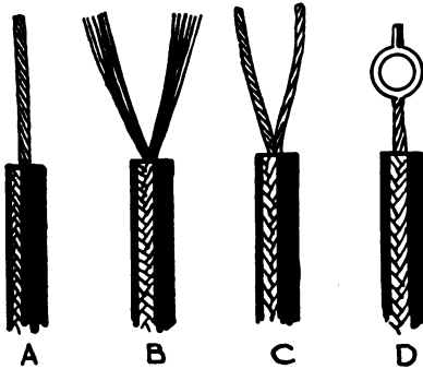
FIG. 327.—Method of making temporary terminals.
