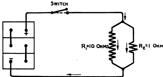
FIG. 7.—Parallel circuits.
