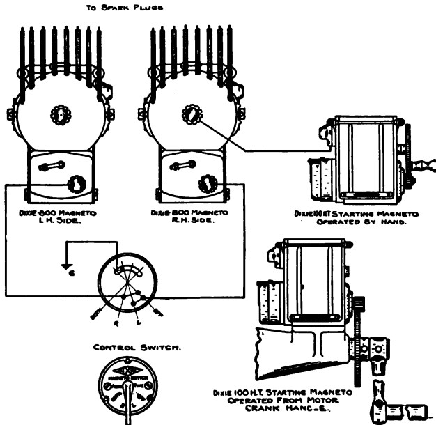
Fig. 303.—External wiring diagram of Aero model 800 ignition system for aircraft with hand starting magneto.
