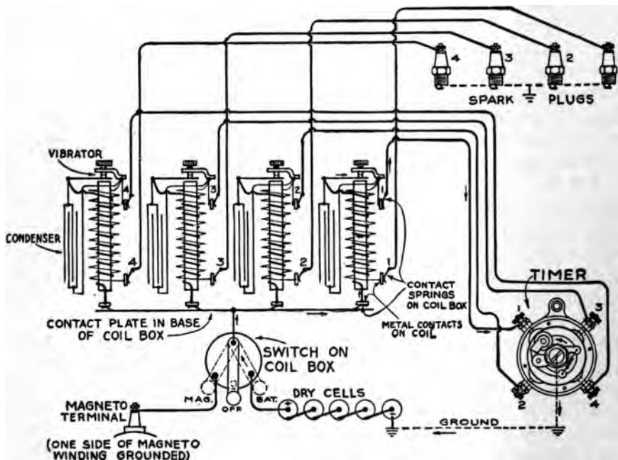
FIG. 83.—Diagram of four-cylinder vibrating coil ignition system.
