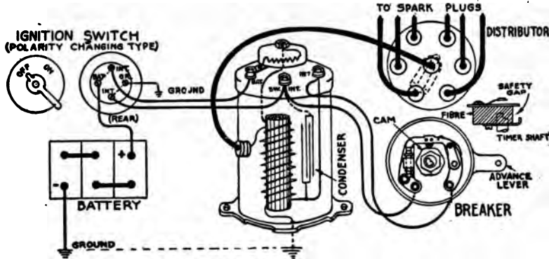
FIG. 123.—Wiring diagram for Remy battery ignition system using three primary terminal coil.
