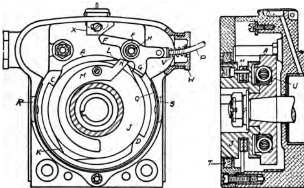
FIG. 290.—Sectional view of Aero impulse starter.
