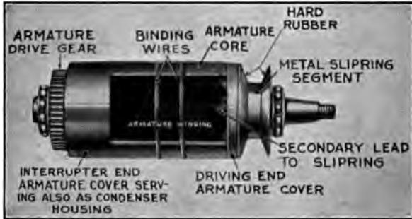
FIG. 203.—View of armature of Bosch DU4 high-tension magnetos showing ball bearing on armature shaft, and pinion that drives distributor gear.
