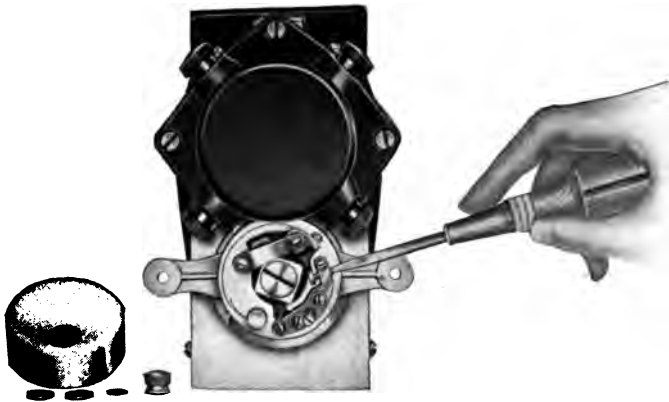
FIG. 275.—Adjusting contact joints, Dixie magneto odel 46.
