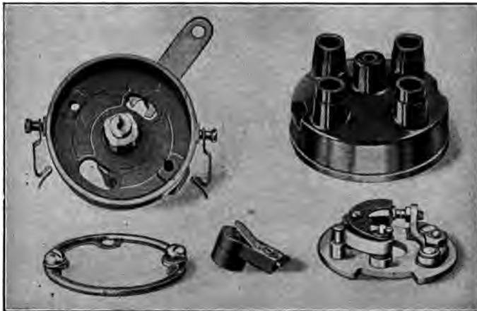
FIG. 113.—Connecticut igniter with distributor head removed showing breaker mechanism, models 16 and 16C.
