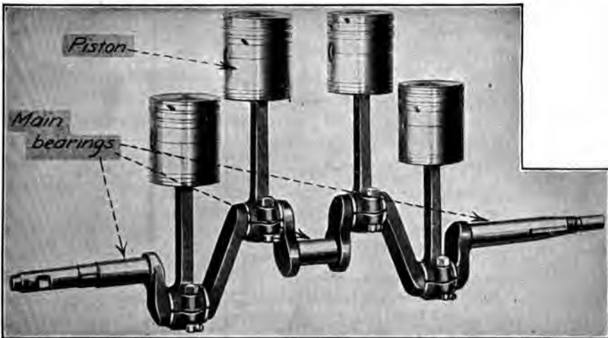
FIG. 150.—Four-cylinder crankshaft.
