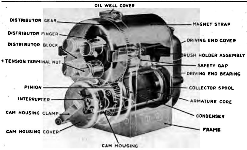
FIG. 241.—X-ray view of Berling high-tension independent magneto.
