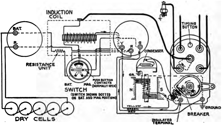
FIG. 196.—Internal circuit diagram of Remy magneto, model RL.
