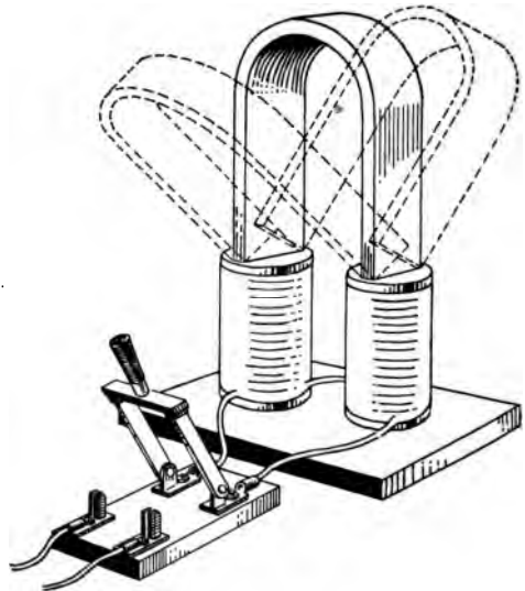
FIG. 340.—Magnet recharger.
