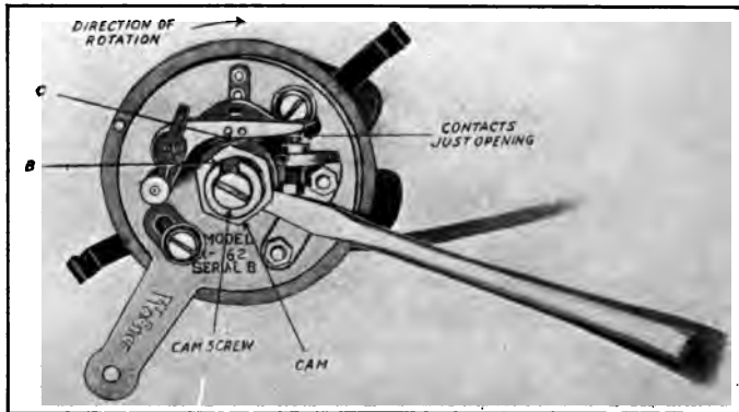
FIG. 149 h .—Timing the Wagner interrupter.
