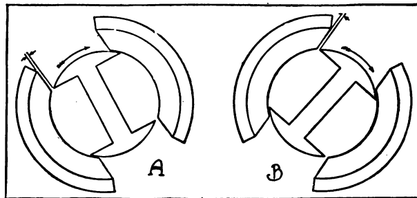
FIG. 248.—Mea magneto—relative position of armature and magneto at the moment of sparking.
