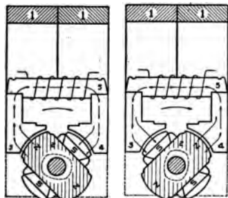
FIGS. 279 and 280.—Reversal of magnetic flux through the coil in Aero magneto.
