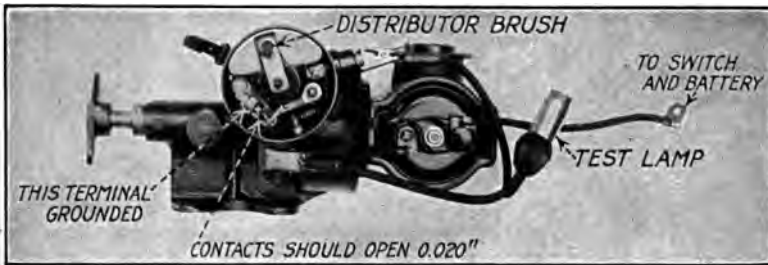
FIG. 130.—Method of connecting test lamp to check time of contact opening.
