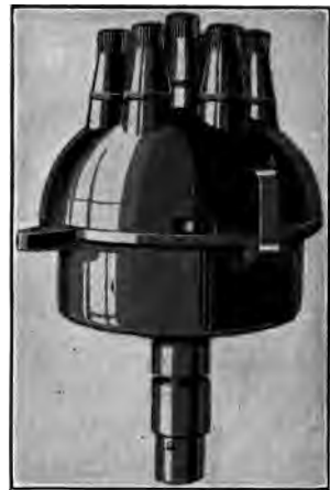
FIG. 94.—Atwater-Kent Unispark, Type K-2.
