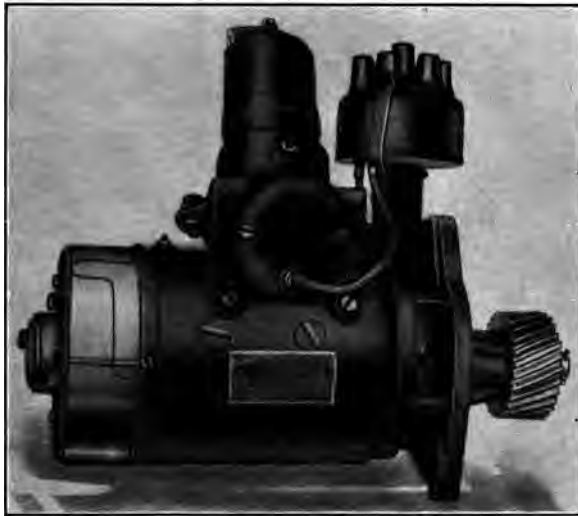
FIG. 149a.—Wagner ignition system mounted on generator.
