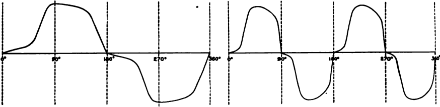
FIG. 258.—Current waves of the rotating armature type magneto.
