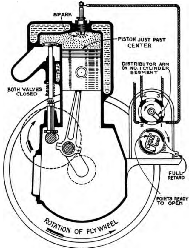
FIG. 320.—Timing the magneto to the engine.
