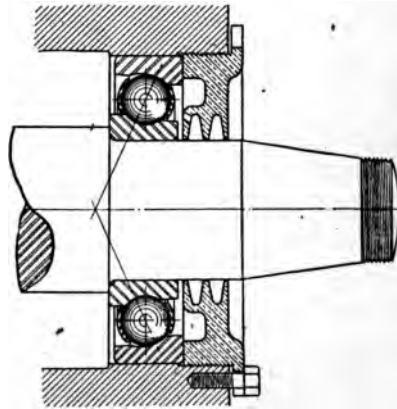
FIG. 318.—Cross section of magneto ball bearing showing angular contact.
