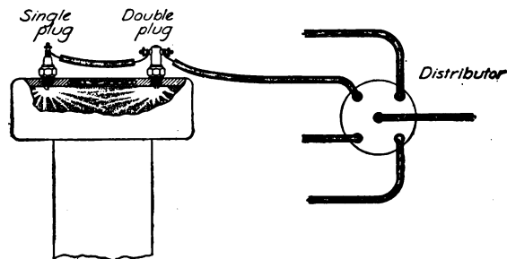
FIG. 88.—Series plug ignition system.
