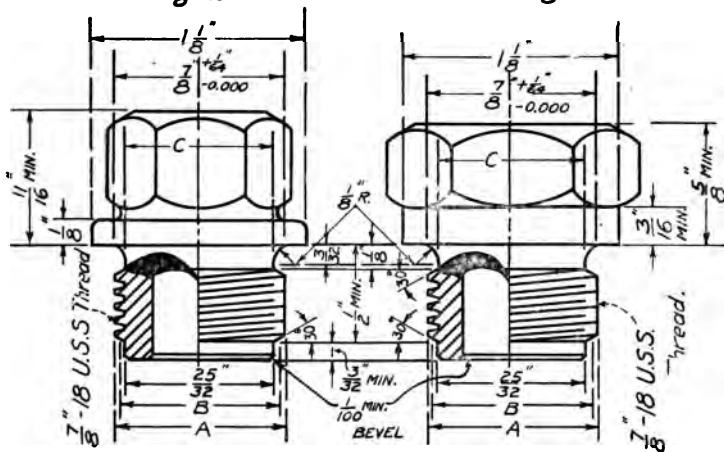
FIG. 79.—Spark plug shell dimensions.
