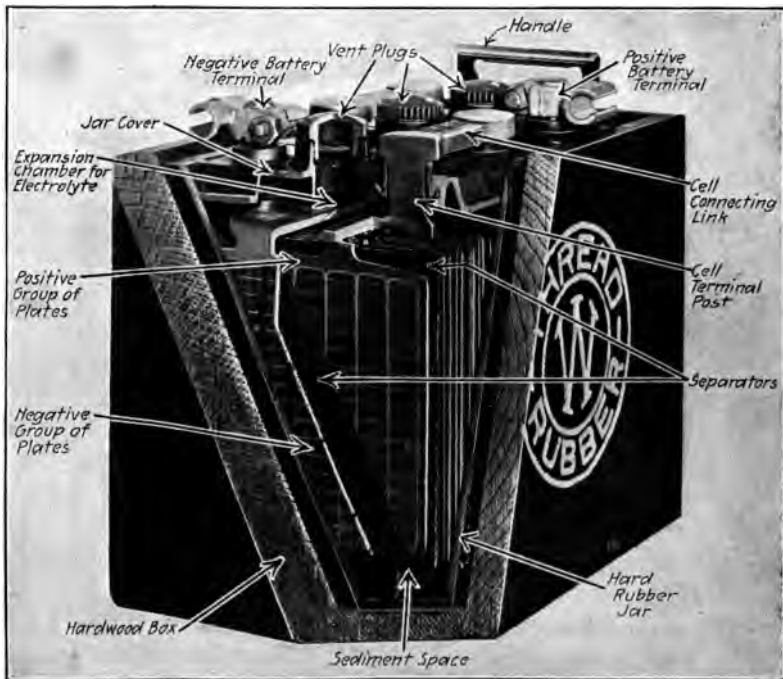
FIG. 41.—Section of typical lead storage battery.
