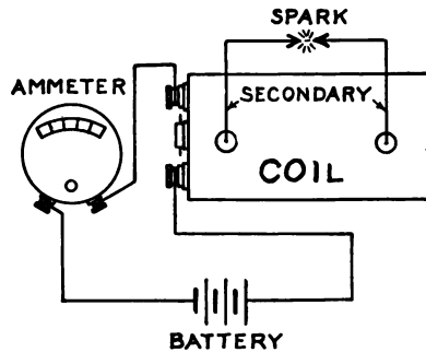
FIG. 333.—Testing vibrating ignition coil.
