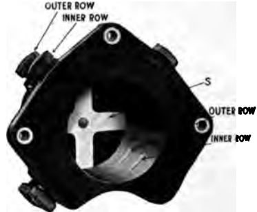
FIG. 295.—Aero eight-cylinder distributor.
