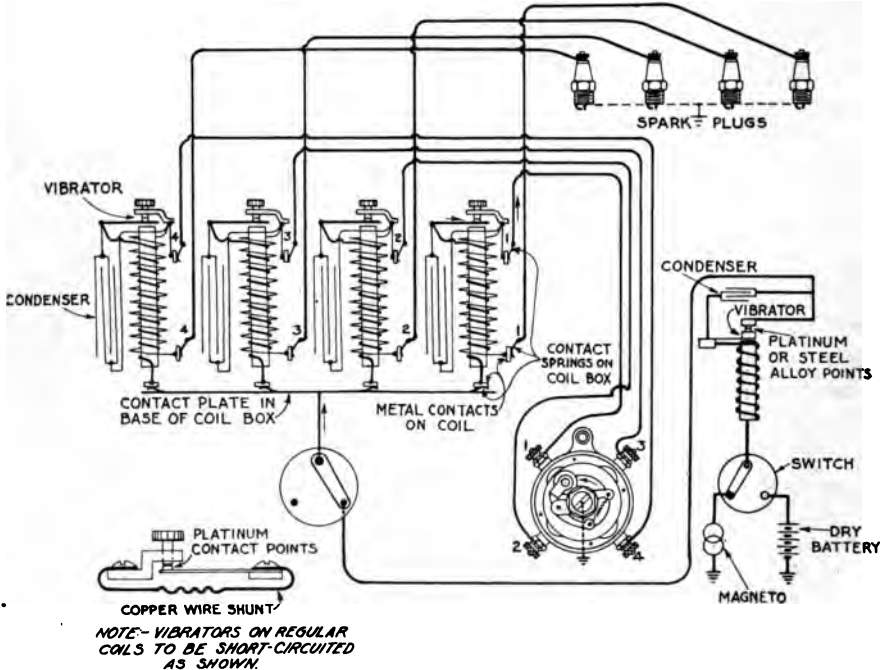
FIG. 87.—Wiring diagram of four-cylinder ignition system using master vibrator in connection with four vibrating type coils.
