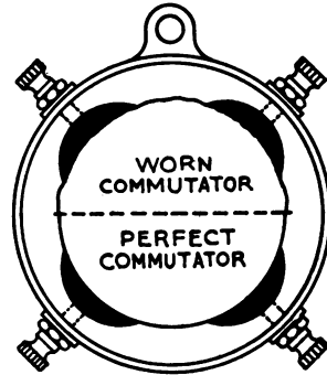
FIG. 322.—Conditions causing interrupter trouble.
