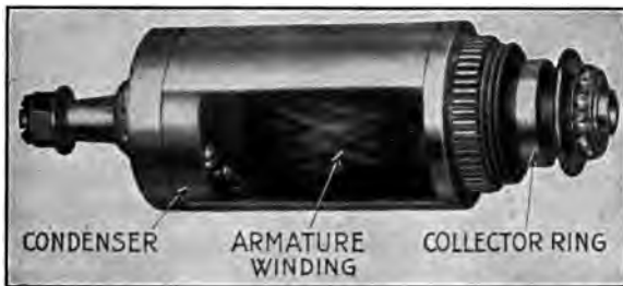
FIG. 226.—Armature for Eisemann magneto.
