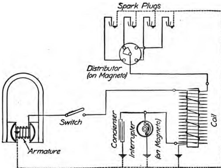
FIG. 185.—Low-tension magneto ignition system with interrupted primary current.
