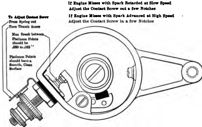
FIG. 193.—Circuit breaker of Remy magneto.
