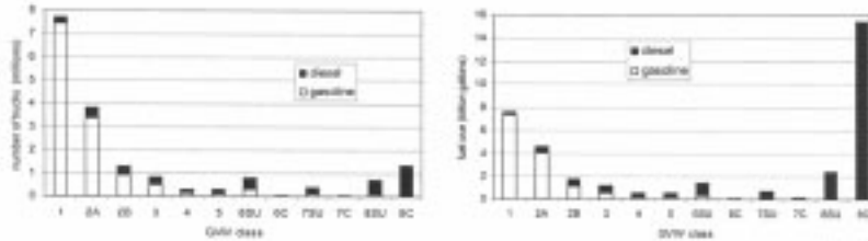
The graph on the left shows the number of commercial trucks (Classes 1-8) in use; the graph on the right shows their fuel use (courtesy of Oak Ridge National Laboratory, 2005)
