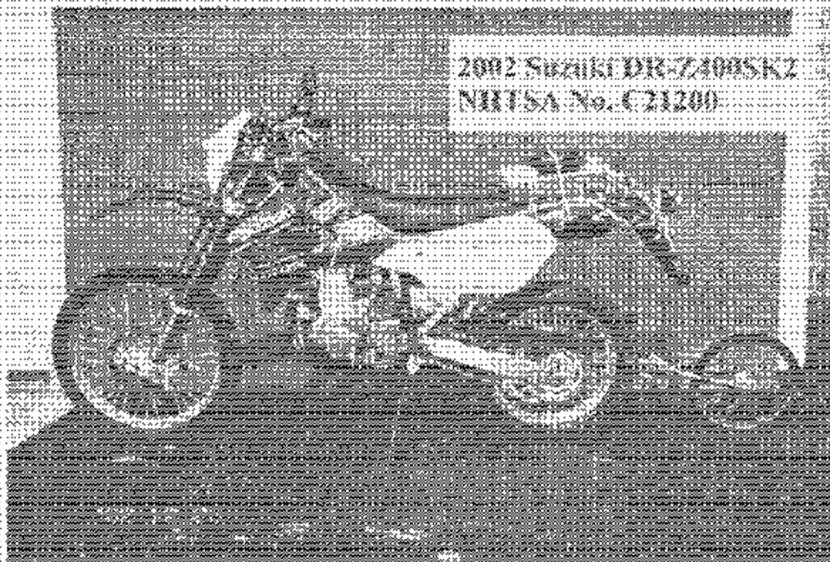
Photograph 2. Left Side View of the Test Motorcycle with Instrumentation Installed.
