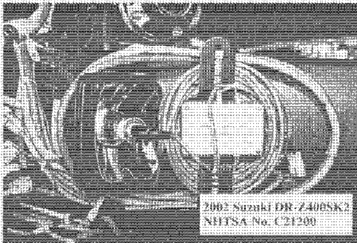
Photograph 9. Brake Application Relay and Tailight Plug-in.
