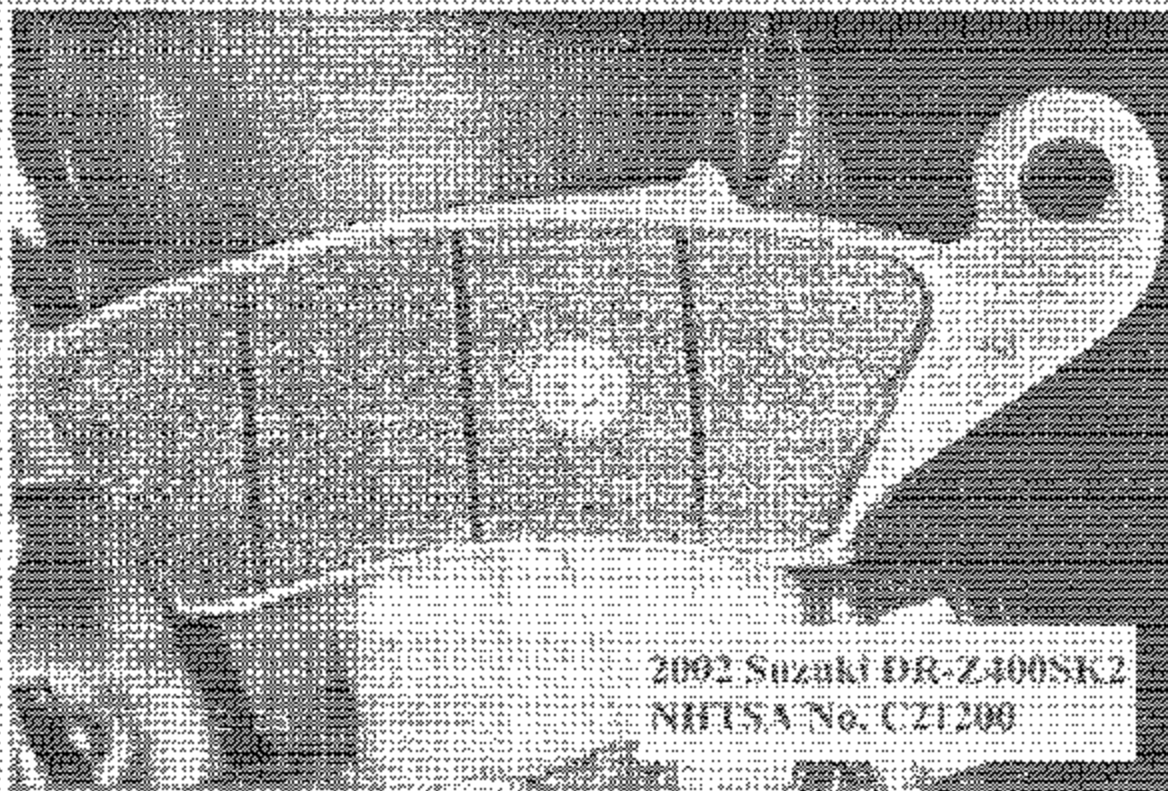
Photograph 14. Typical Disk Brake Pad Thermocouple Installation (Post-Fest).
